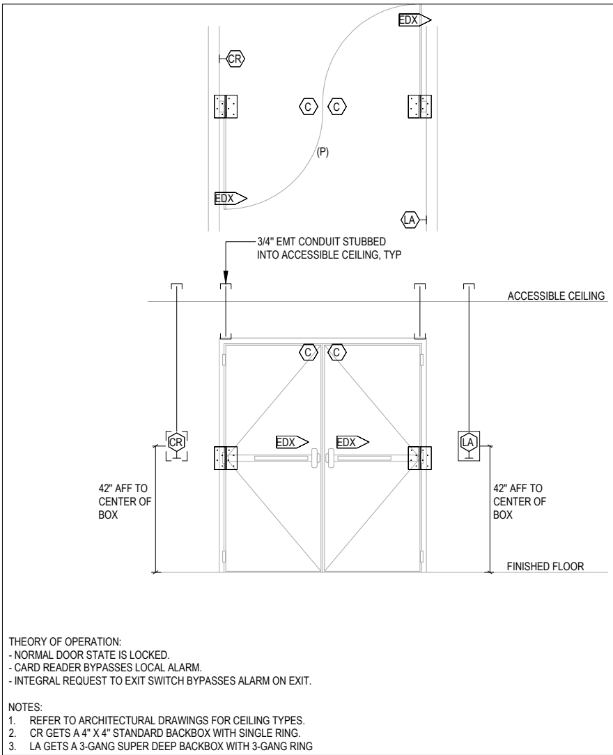
DOUBLE DOOR - EXIT DEVICE, CARD READER, S DOOR
