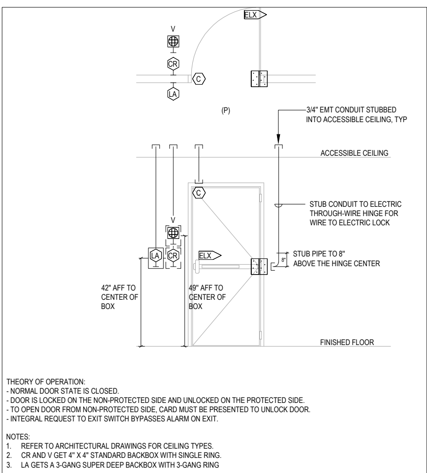
SINGLE DOOR - ELECTRIC LOCK, CARD READER, INTERCOM
