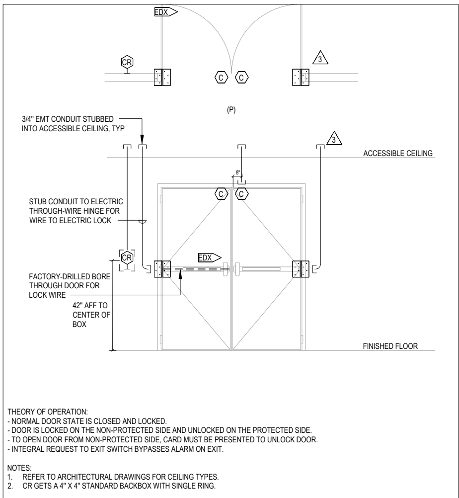
DOUBLE DOOR - EXIT DEVICE, CARD READER
