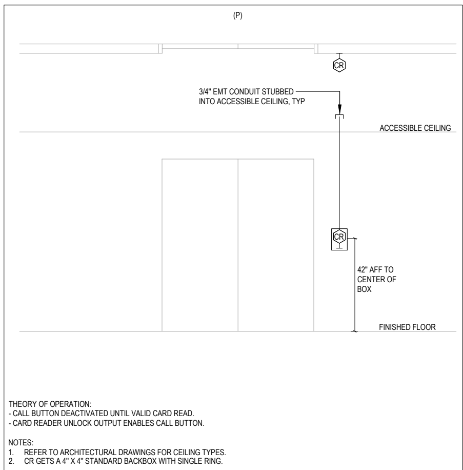
CARD READER - ELEVATOR HALL
