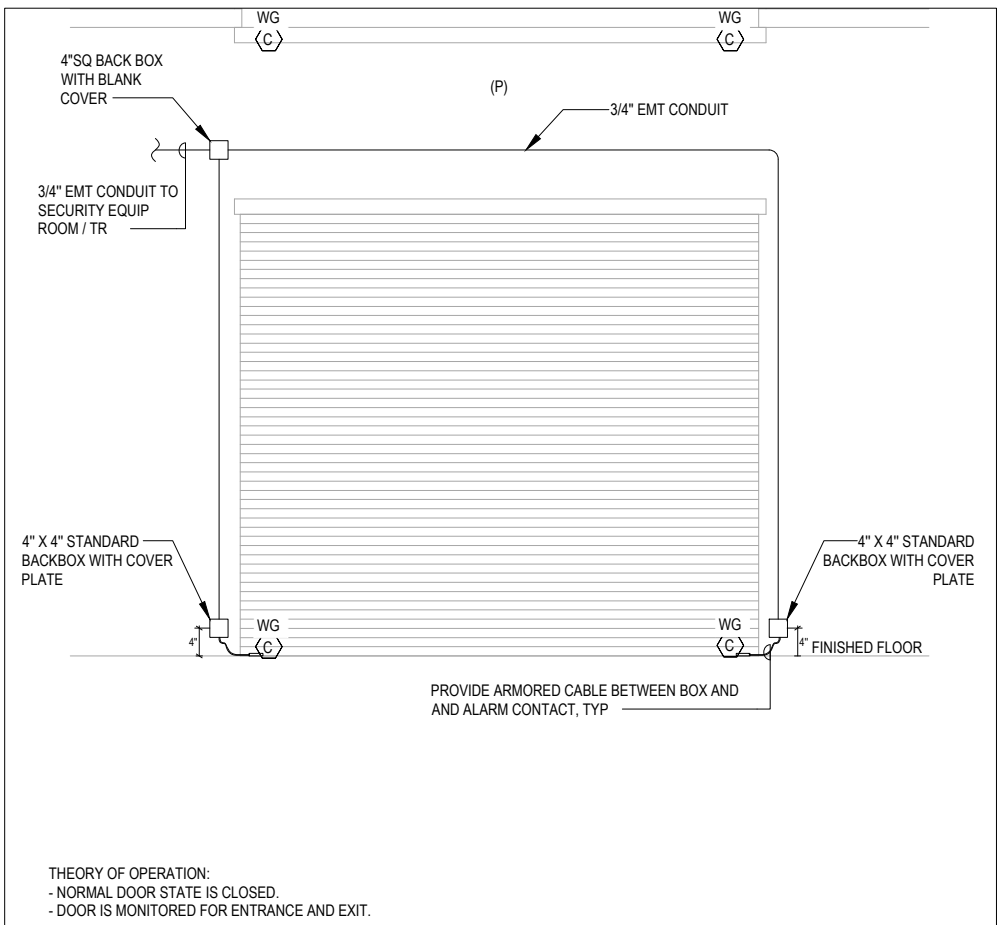
COILING DOOR - MONITORED
