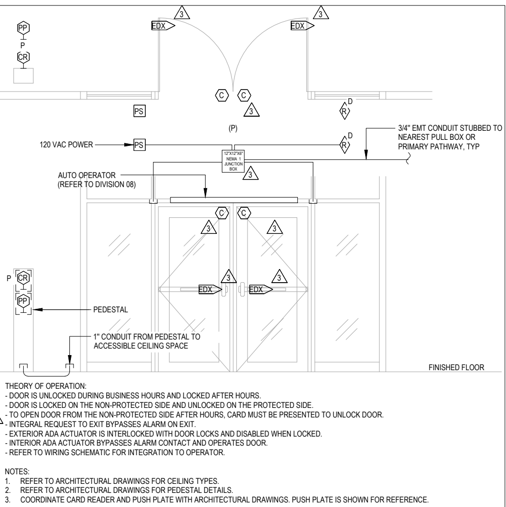
DOUBLE DOOR - AUTO-OPERATOR, CARD READER
