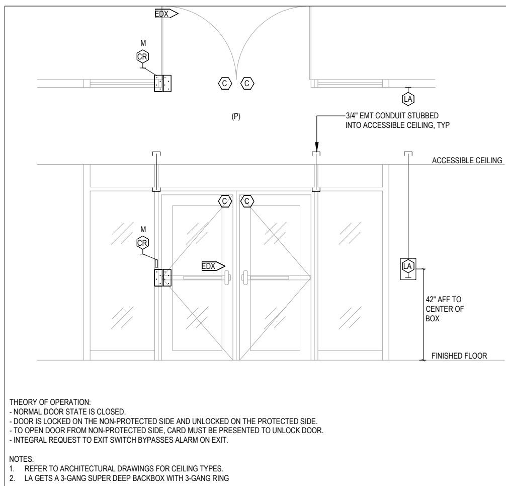
DOUBLE DOOR - EXIT DEVICE, CARD READER, LOCAL ALARM
