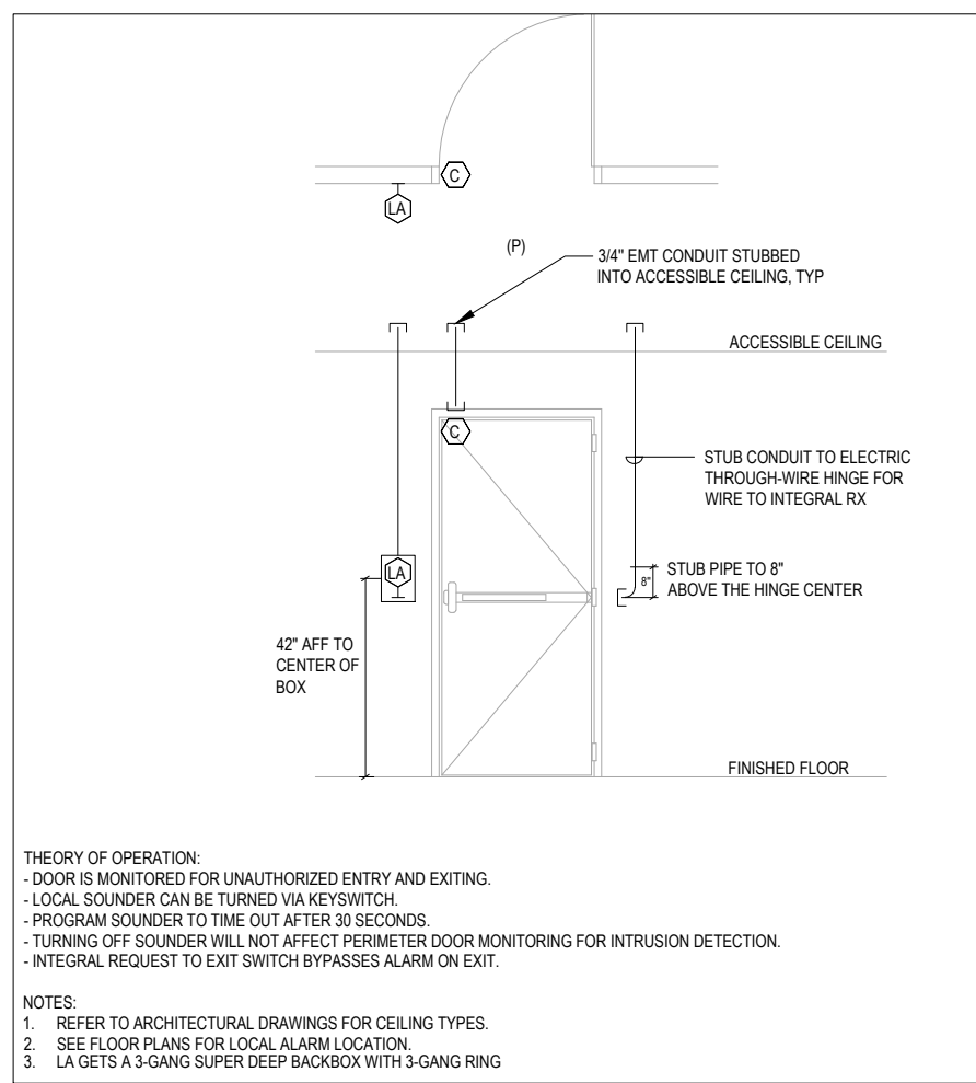
SINGLE DOOR - ALARM MONITORED, LOCAL ALARM
