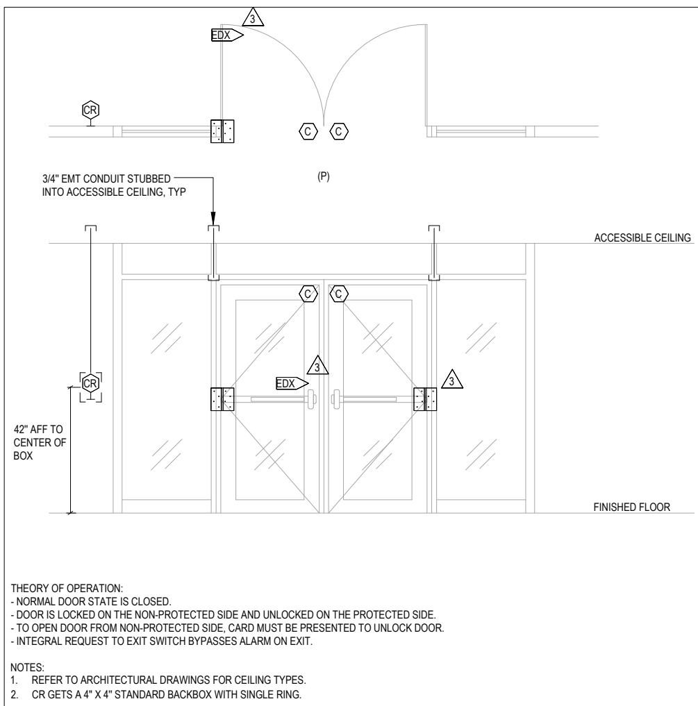
DOUBLE DOOR - EXIT DEVICE, CARD READER
