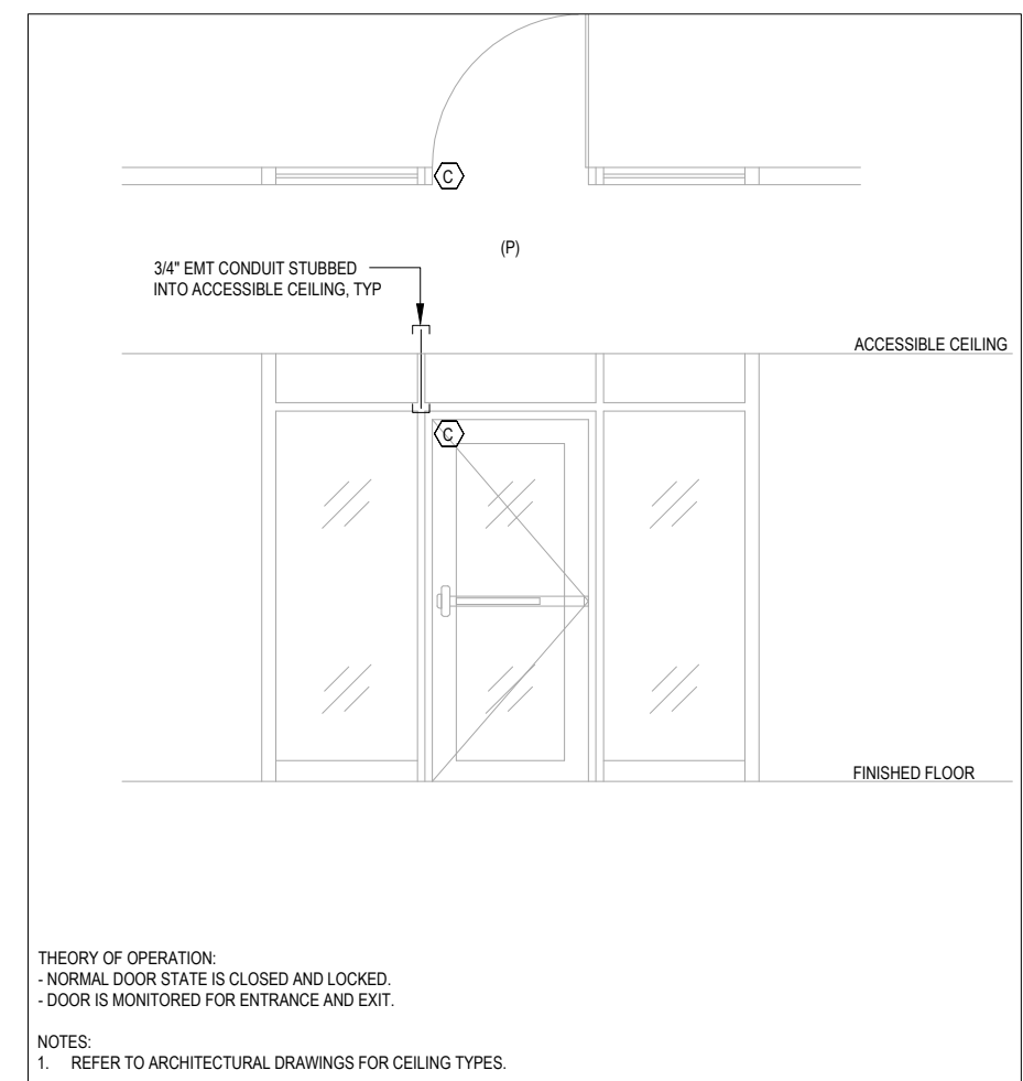
SINGLE DOOR - EXIT DEVICE, MONITORED
