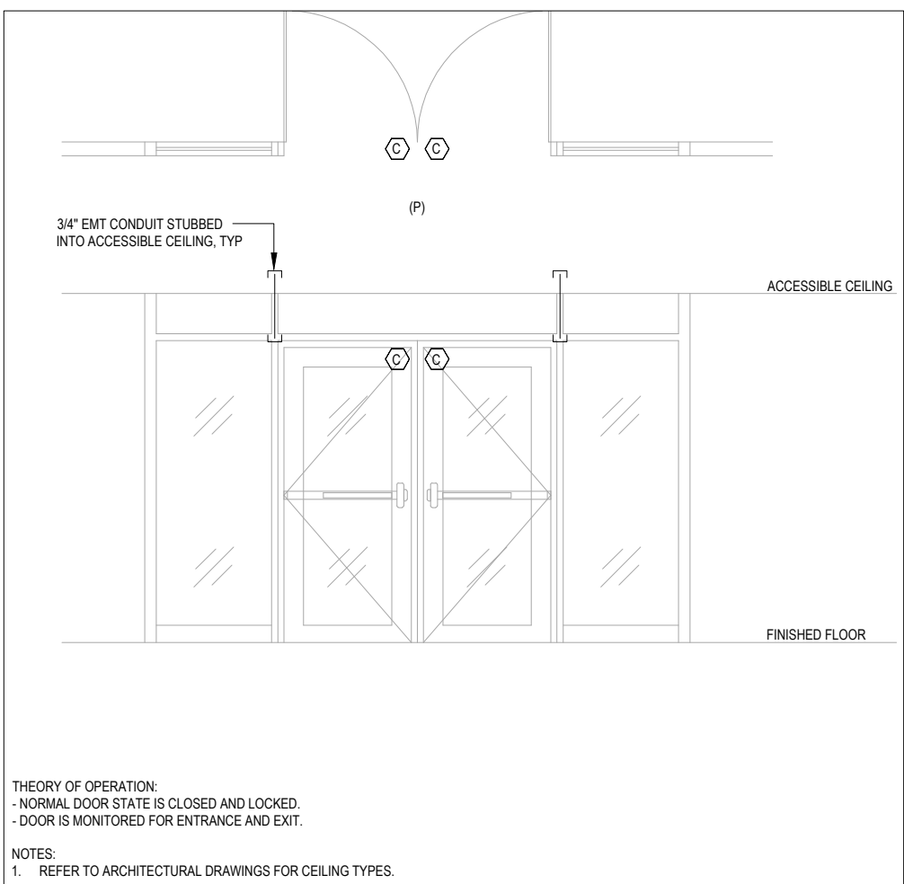
DOUBLE DOOR - EXIT DEVICE, MONITORED
