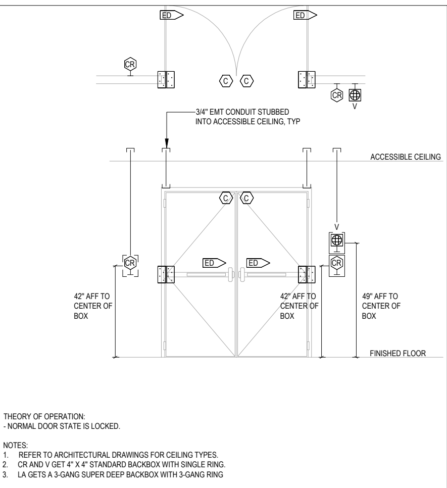
DOUBLE DOOR - EXIT DEVICE, CARD READER PAIR, INTERCOM
